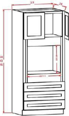
OVEN Cabinet Split Doors
