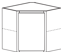
Wall Corner Angle Cabinet, Single Door
